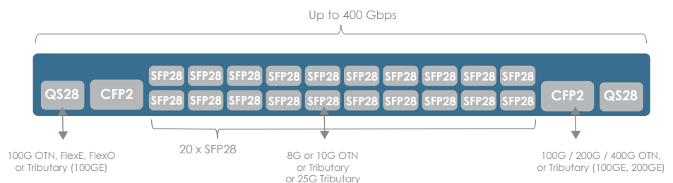
Figure 1: PM_LC4-MP2-A Interfaces
