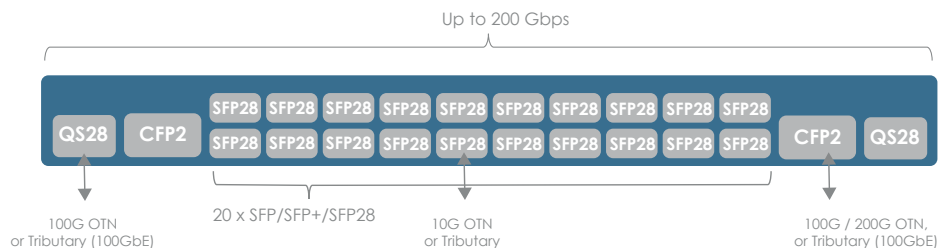
Figure 1: PM_LC4-MP2-A Interfaces
